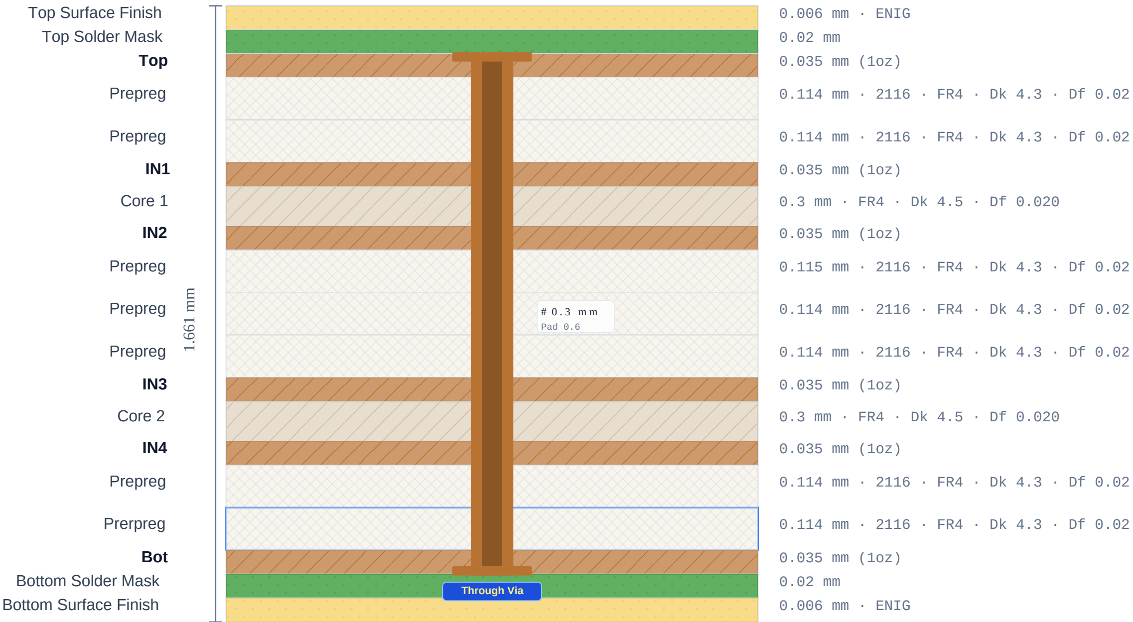
6 Layer 1.6mm 35µm Stackup
